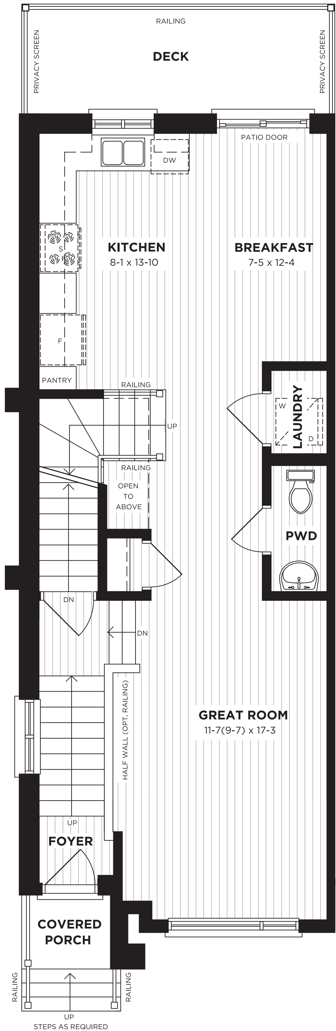
MAIN FLOOR
