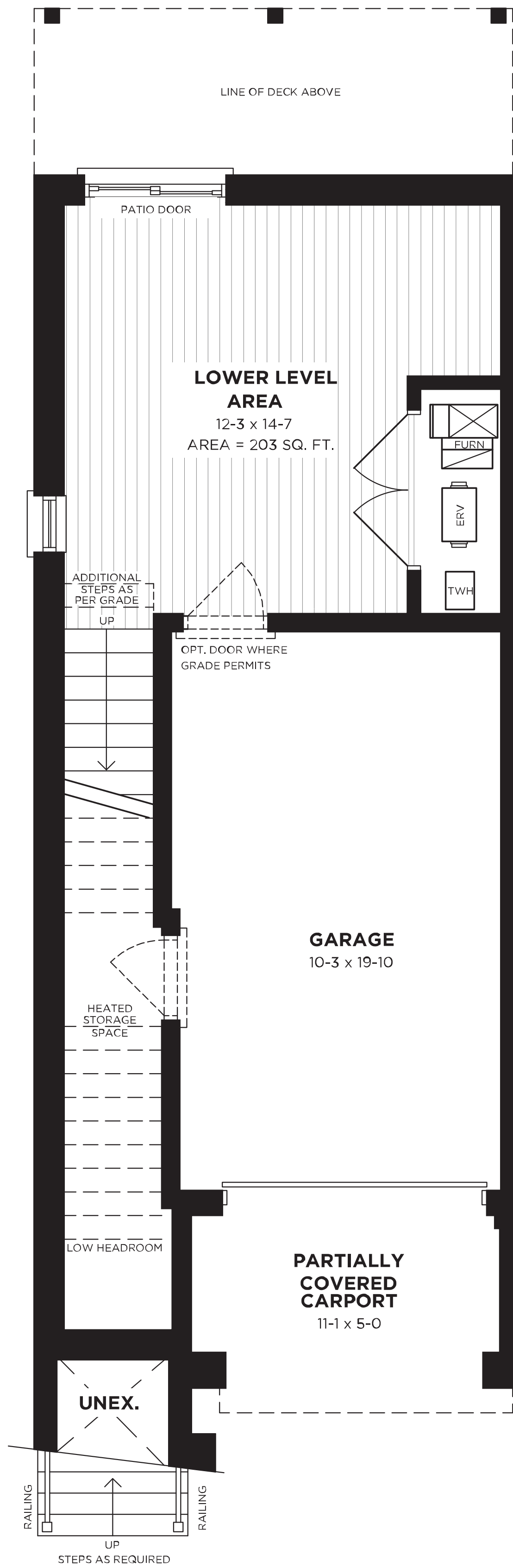
GROUND FLOOR
