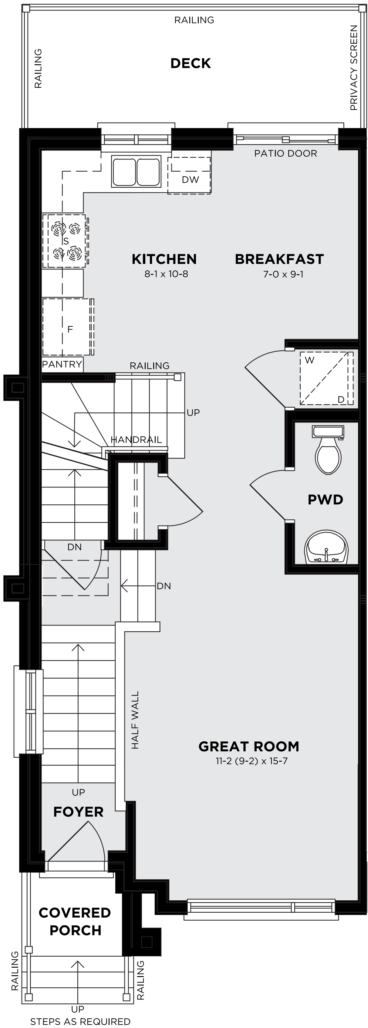
MAIN FLOOR
