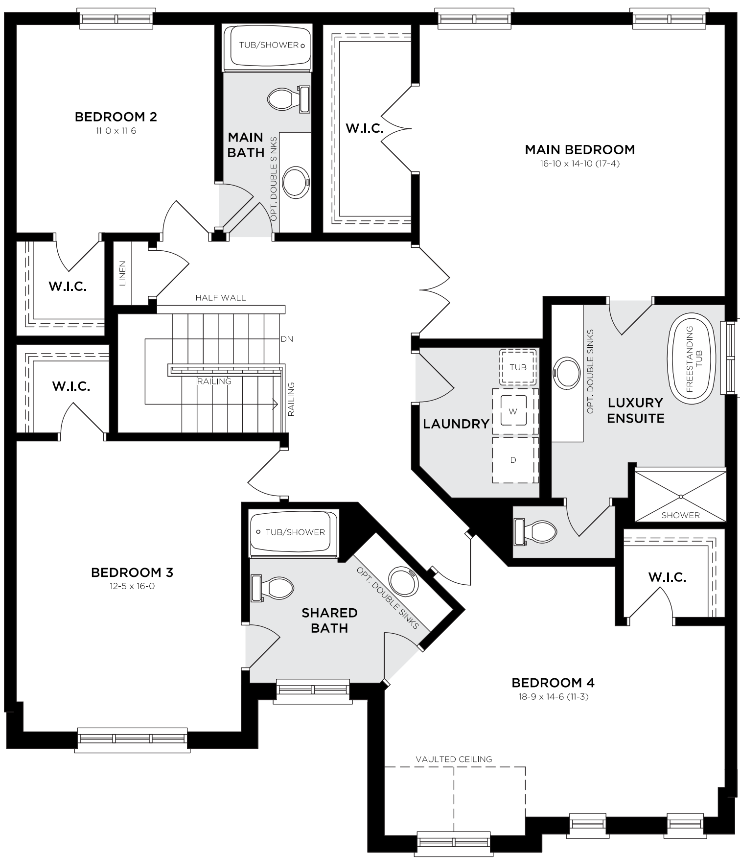
SECOND FLOOR - TRADITIONAL
