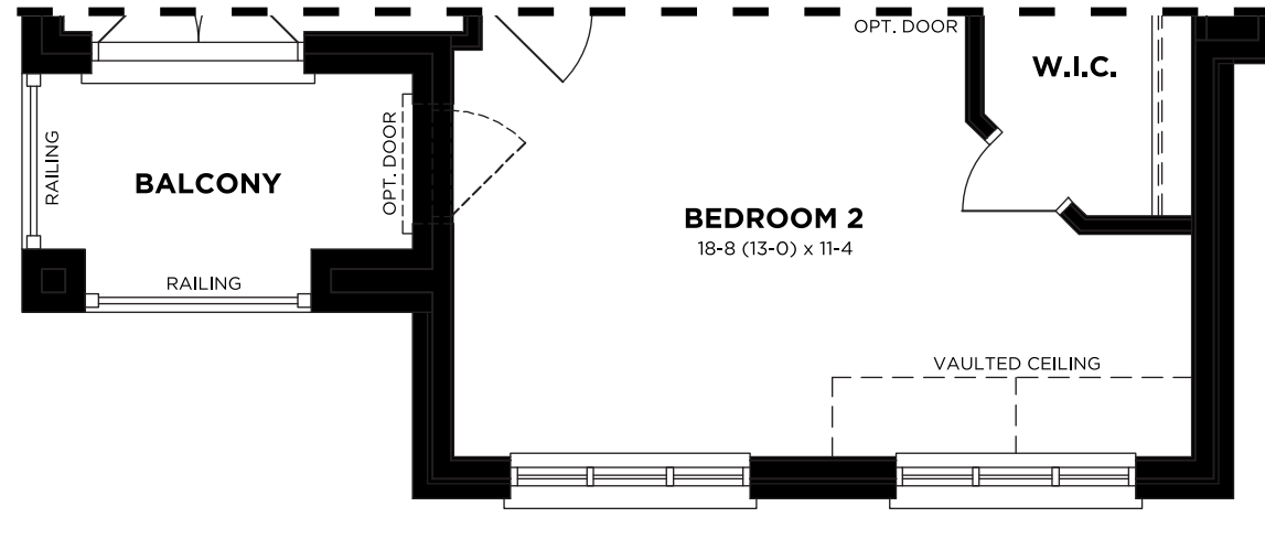
SECOND FLOOR - MODERN
