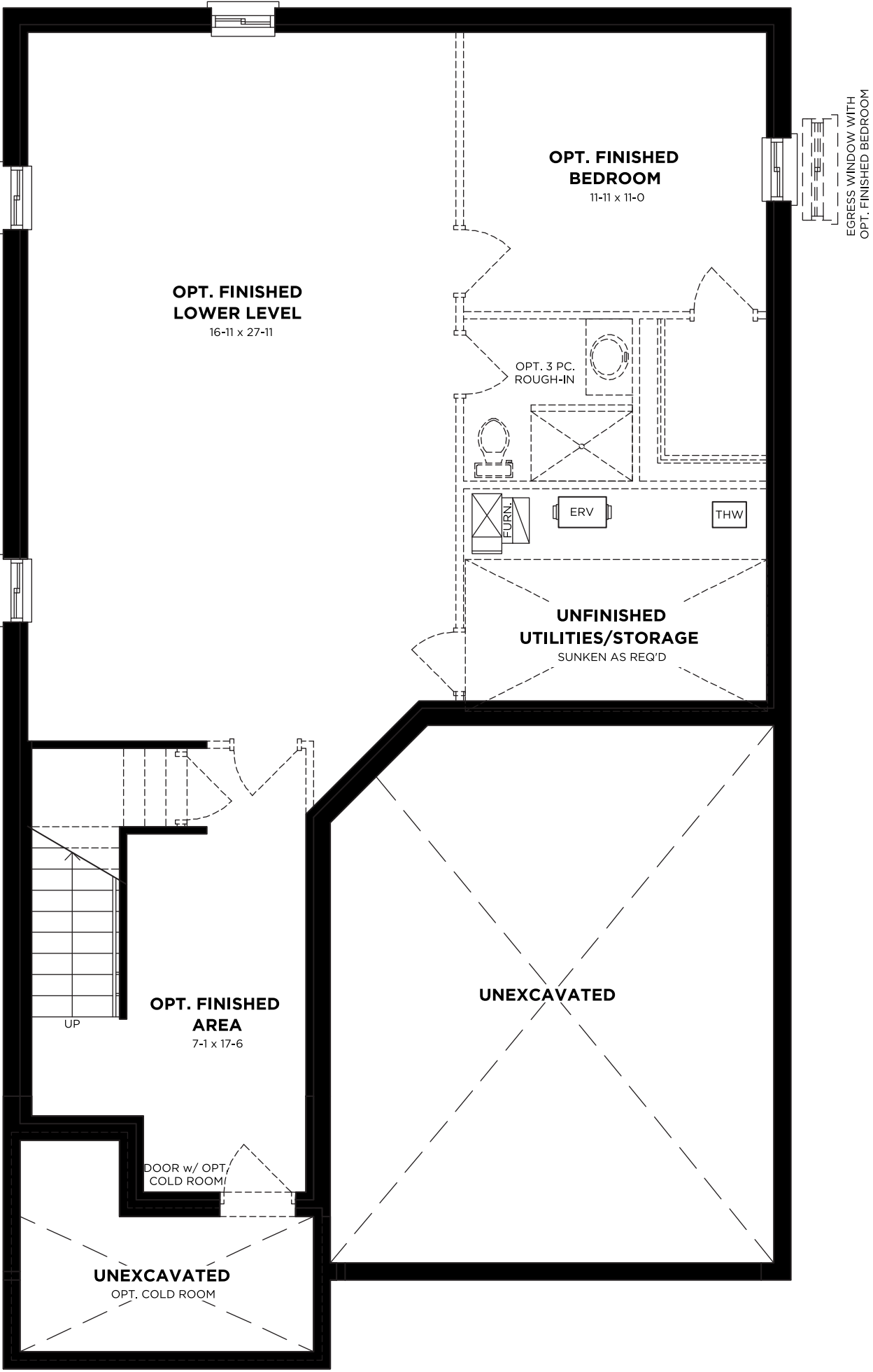
LOWER LEVEL
