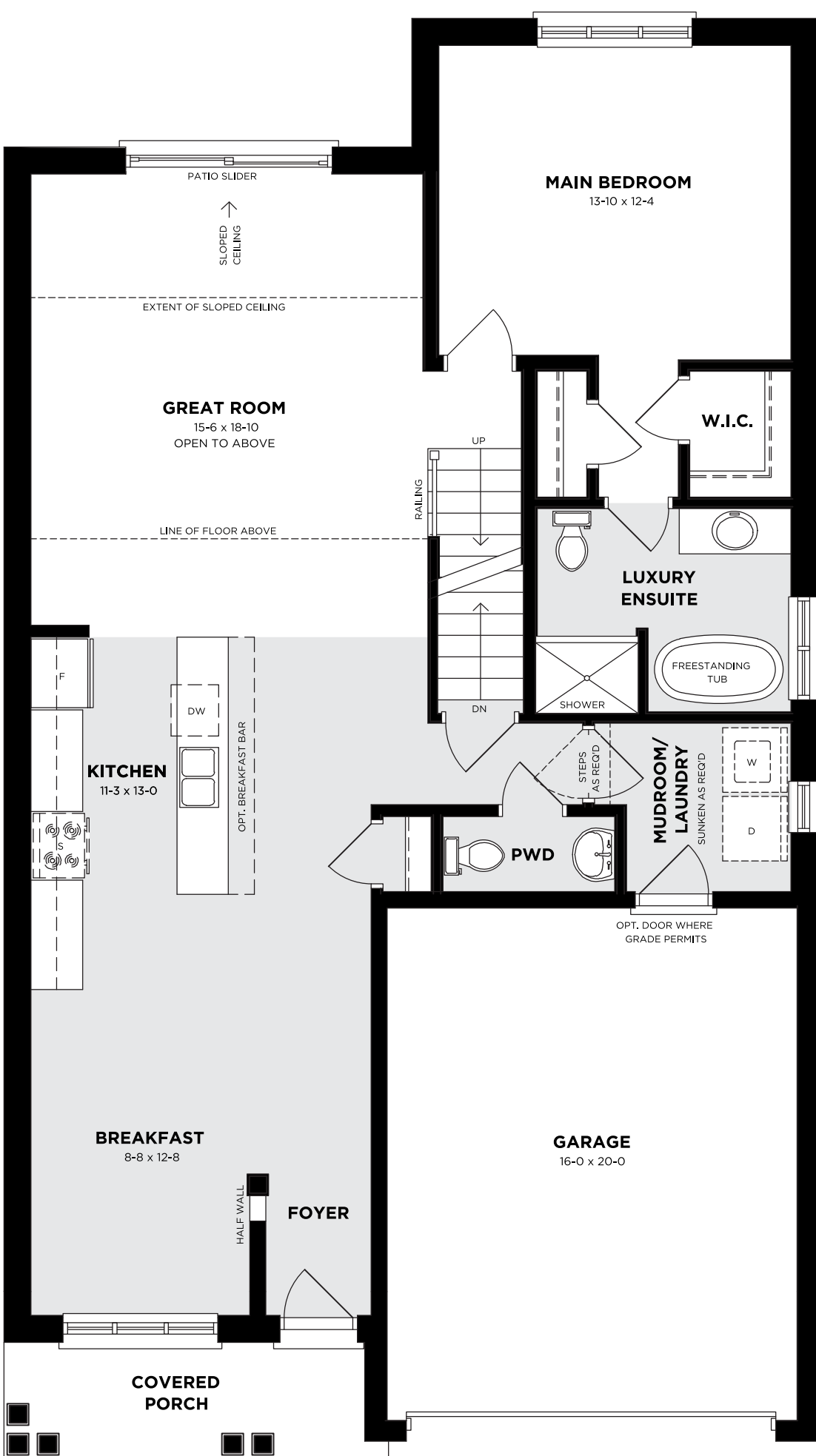
MAIN FLOOR - TRADITIONAL
