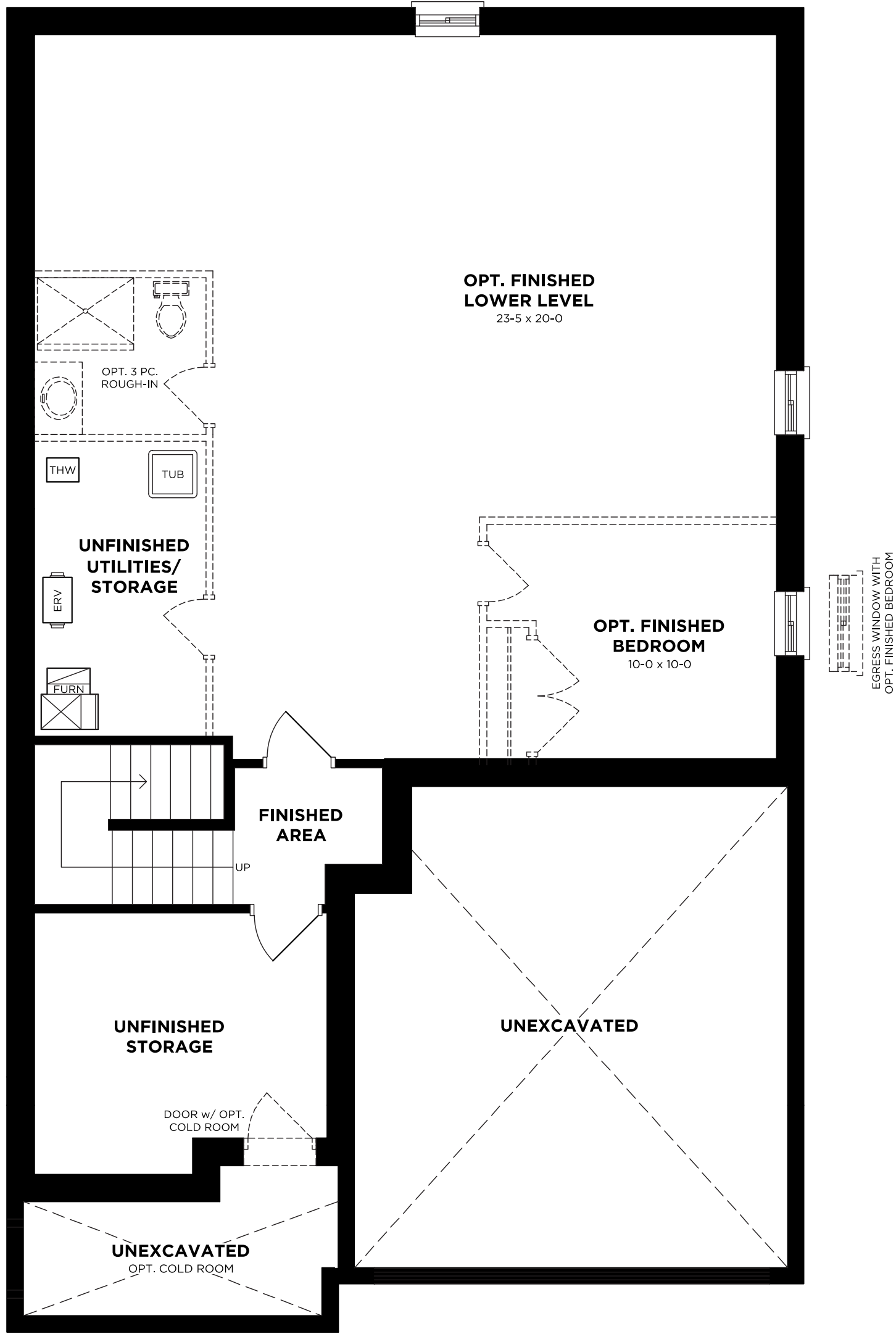
LOWER LEVEL
