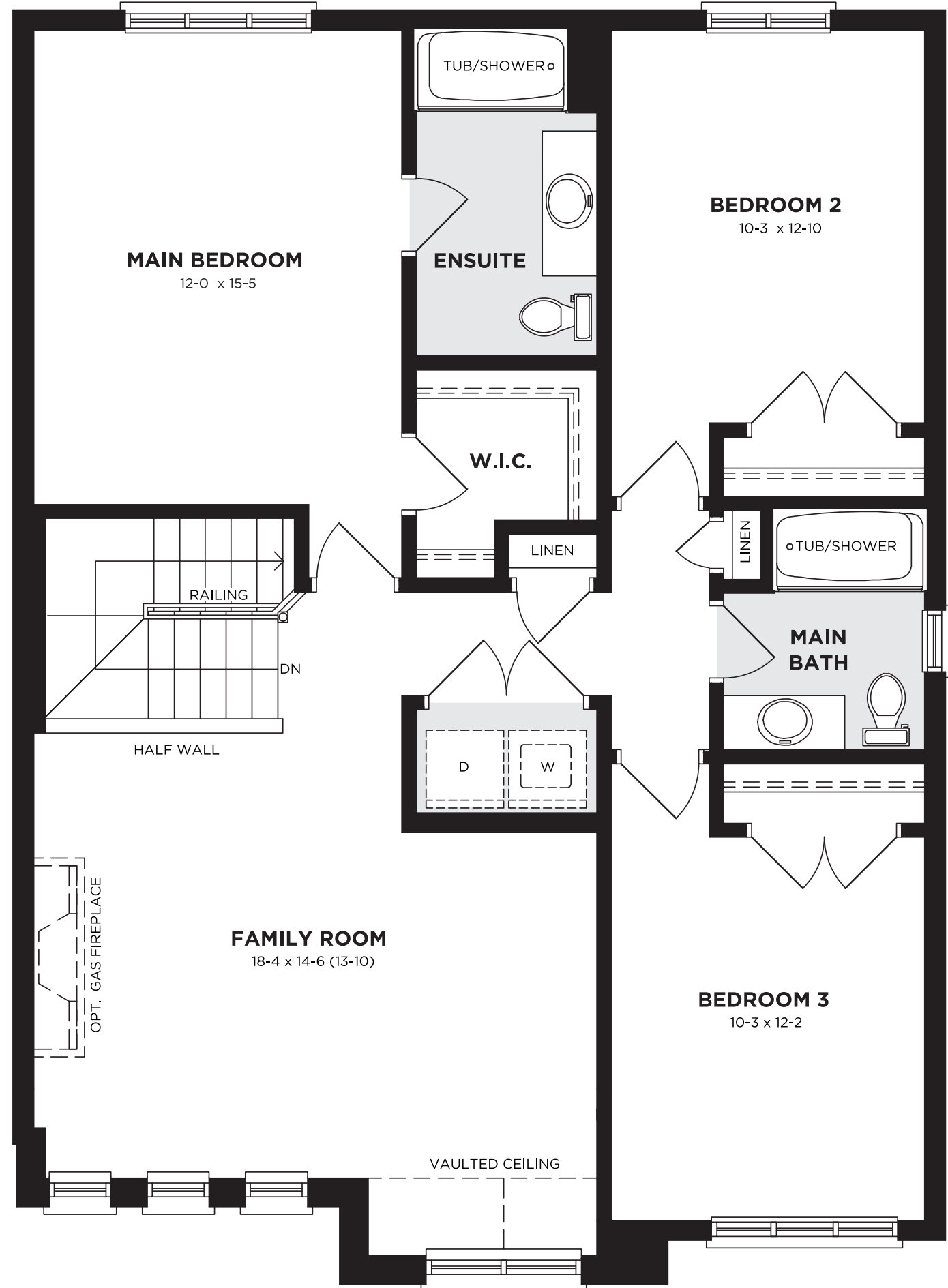
SECOND FLOOR - TRADITIONAL
